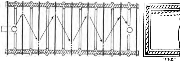
FIG. 302.—Section and End View of an Efficient American Muffler. The muffler consists of a series of chambers formed by screens, perforated alternately at top and base, so that the expanding exhaust gas follows the course indicated by the arrows; their passage through the perforated sections serving to break it up and silence the noise due to its pressure.
